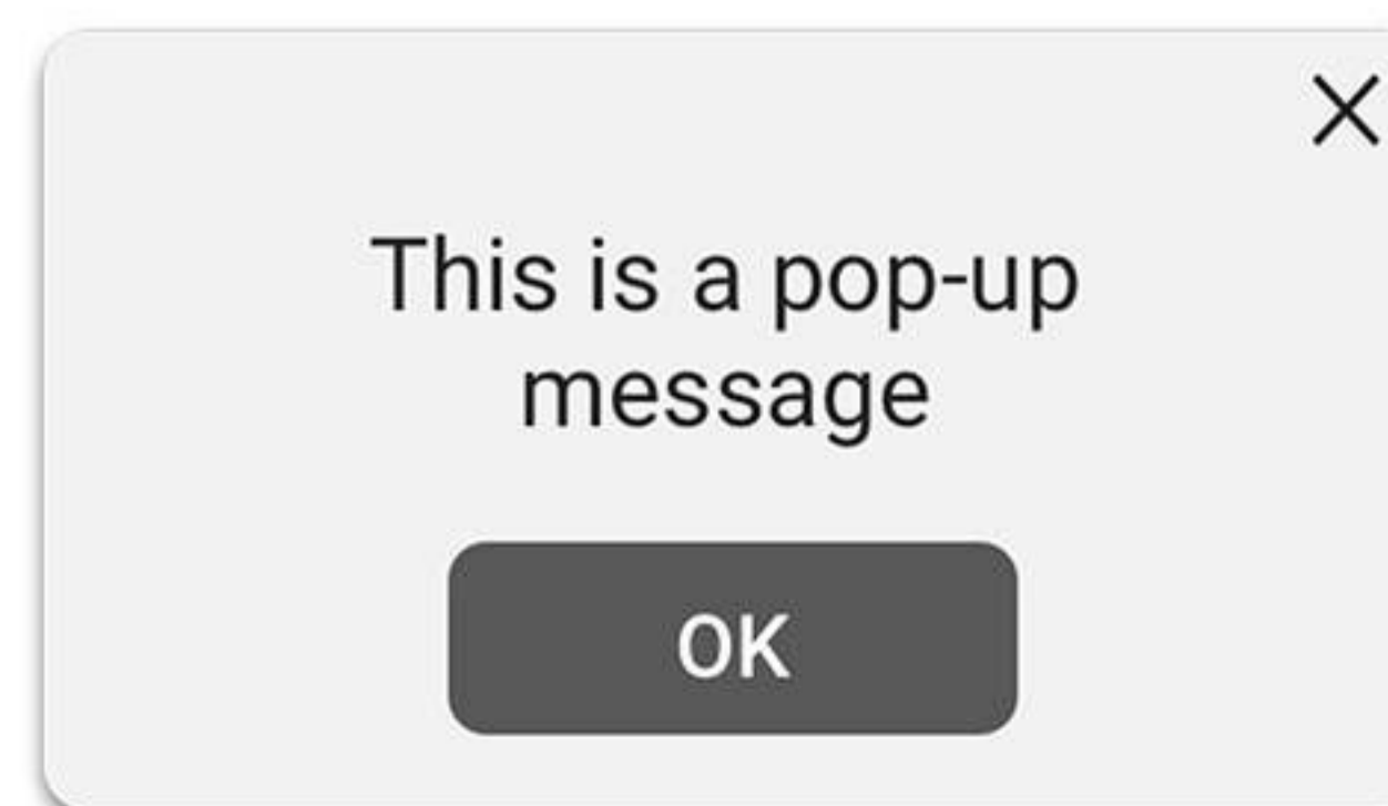
Pop-Up Dialog
