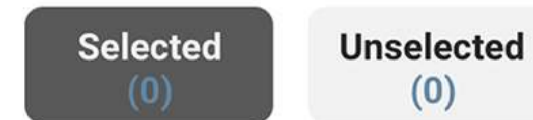
Button States
